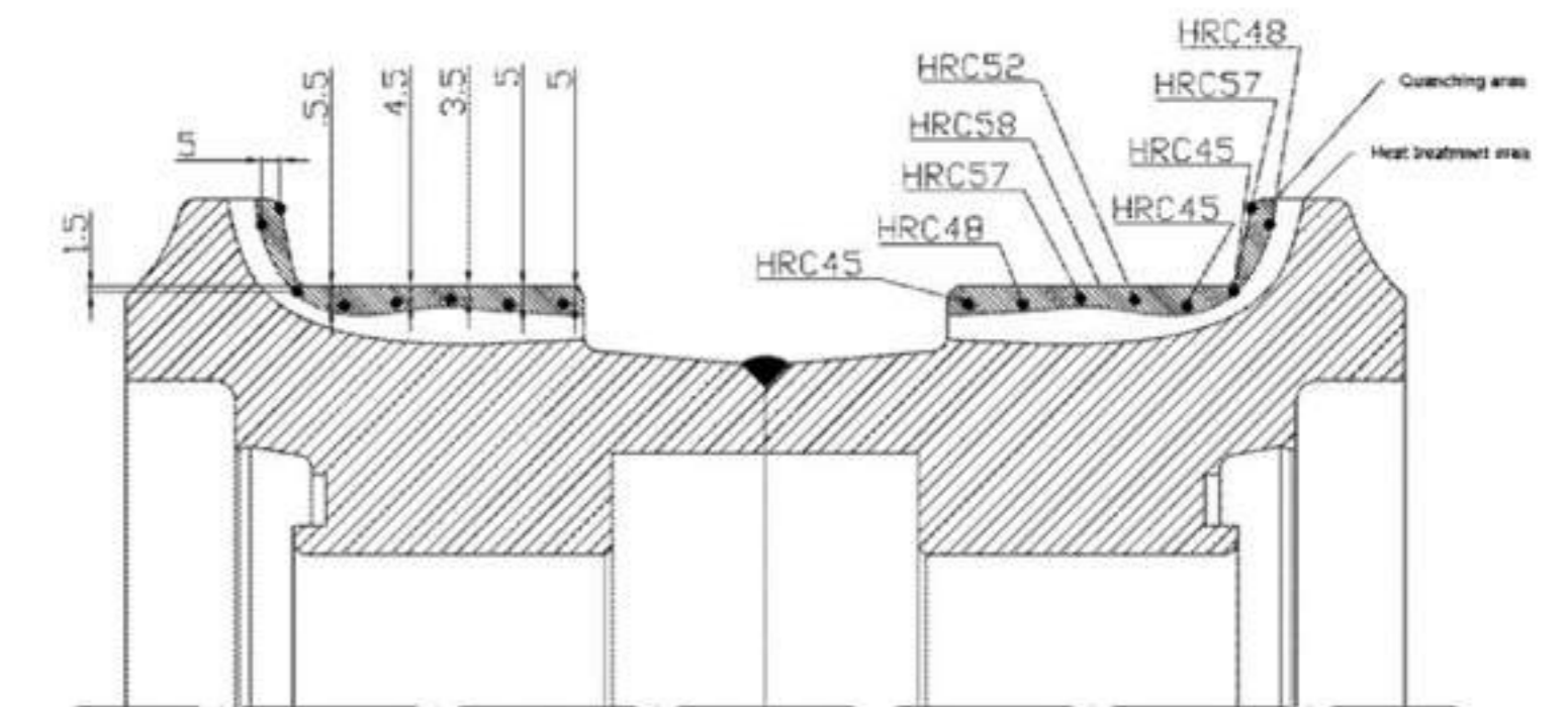
Induction Harden illustration
